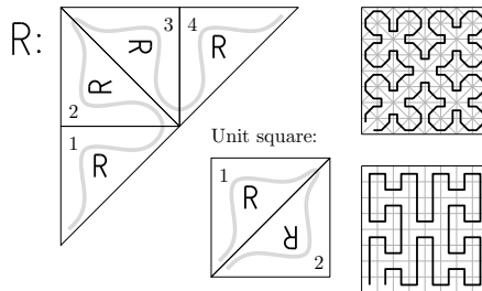
Figure 2: Space-filling curve definitions.
