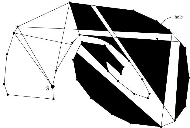
Figure 8: A hole after three specular reflections.
