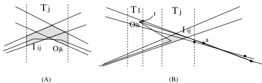
Figure 6: Simple path
