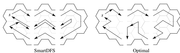
Figure 8: S(P) = \frac{4}{3}S_{\text{Opt}}(P) - \frac{7}{3} holds.
