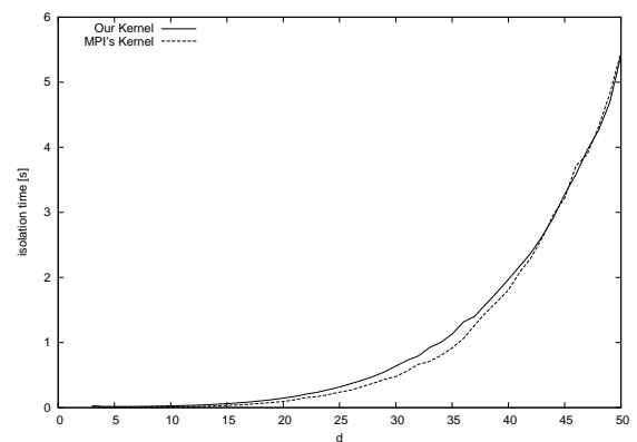
Figure 4: Mignotte polynomials
