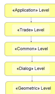
Figure 2: The different abstraction levels.
