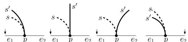
Figure 1: Selecting a seed node if sites meet tangentially.
