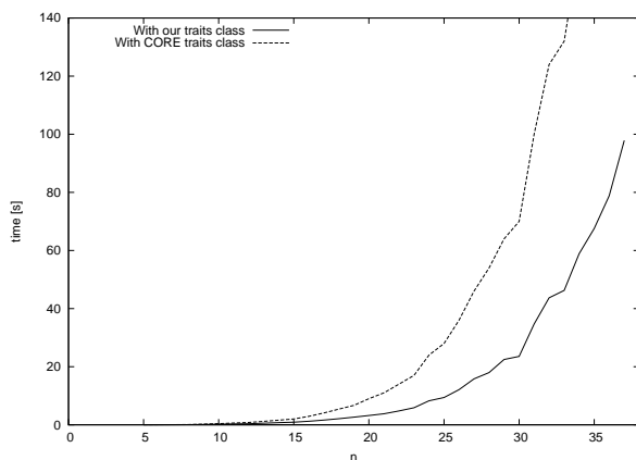
Figure 5: Arrangement calculation
