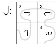
Figure 2: Space-filling curve definitions.
