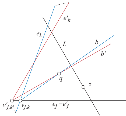
Figure 6: When e'_k rotates to e_k about z , q = b' \cap b is left of L , the perpendicular to b' through z .
