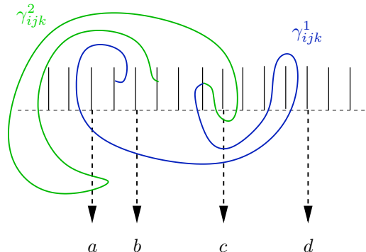
Figure 2: A 3-segment \gamma_{ijk} \in [R] whose pattern with respect to a, b, c and d is (1, 1, 0, 0, 0, 0, 1, 0) , the third entry T_c^1 is 0 because I_c^1(ijk) = 2 \equiv 0 \pmod{2} .
